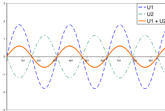
Fig 6: Addition of two correlated voltages, 180° phase angle
