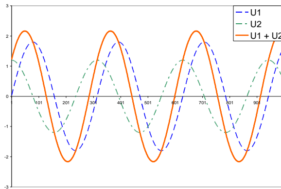
Fig 5: Addition of two correlated voltages, 90° phase angle
