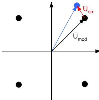
Fig 15: Modulation error
