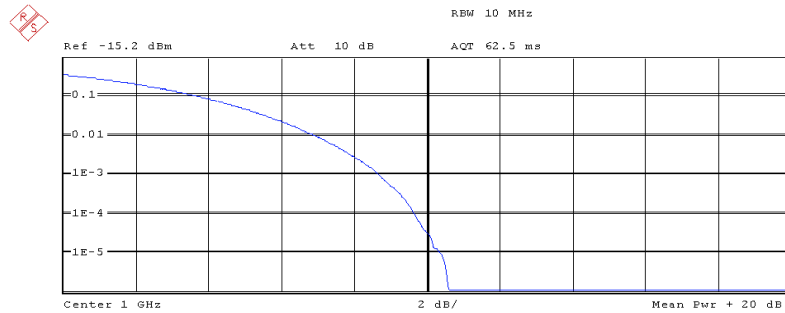
Fig 13: Crest factor measured with the Signal Analyzer R&S® FSQ
