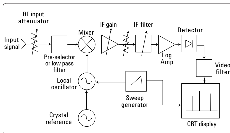
Figure 2-1. Block diagram of a typical traditional superheterodyne spectrum analyzer.
