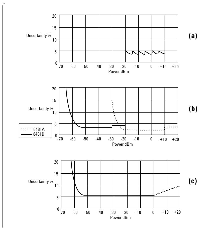
Figure 3-1. RSS uncertainty vs. dynamic power range from data sheet specs for source SWR = 1.15 ( \rho_s = 0.07 ) and f = 2 GHz: (a) Analog thermistor mount system (432A plus 8478B). (b) E4418B digital power meter system using 8481D diode and 8481A thermocouple sensors. (c) E4418B digital power meter and E4412A PDB extended-range sensor. RSS-combining method is the same as used in Fundamentals Part 3 .
