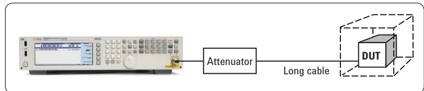
Figure 6b. When decreasing amplitude range, place your DUT in a shielded environment.
